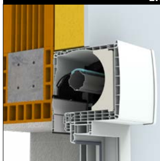
LA SOLUTION VOLET ROULANT A COFFRE APPARENT
